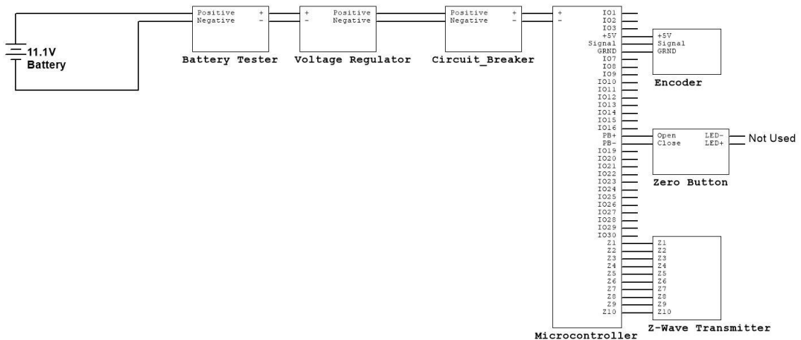
Figure 29: On-Board Schematic
