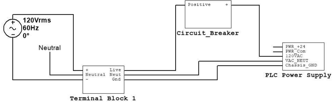
Figure 32: PLC Power Supply Schematic
