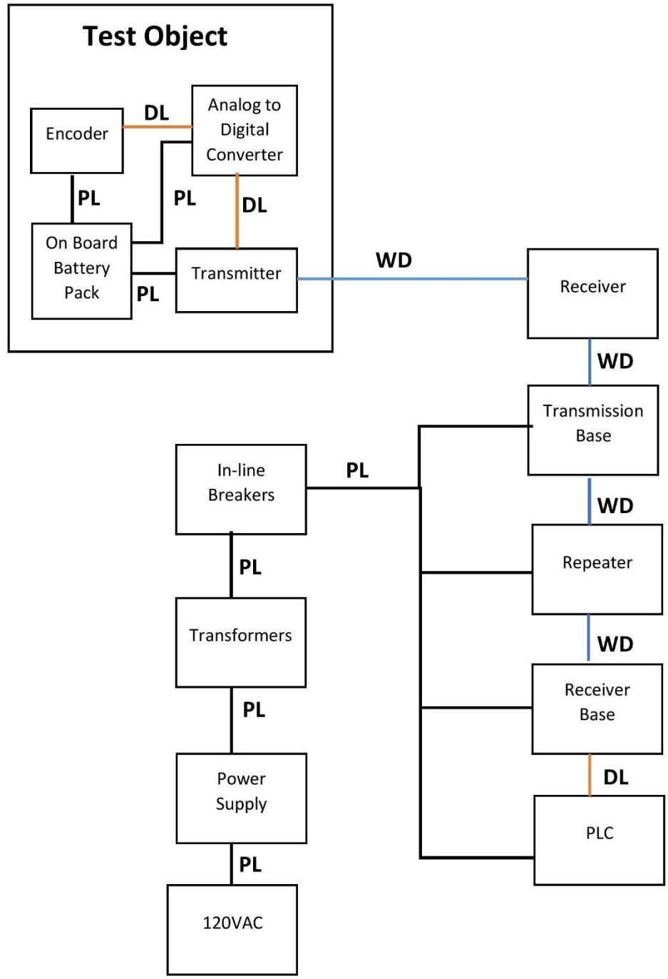
Figure 3: Concept A Block Diagram
