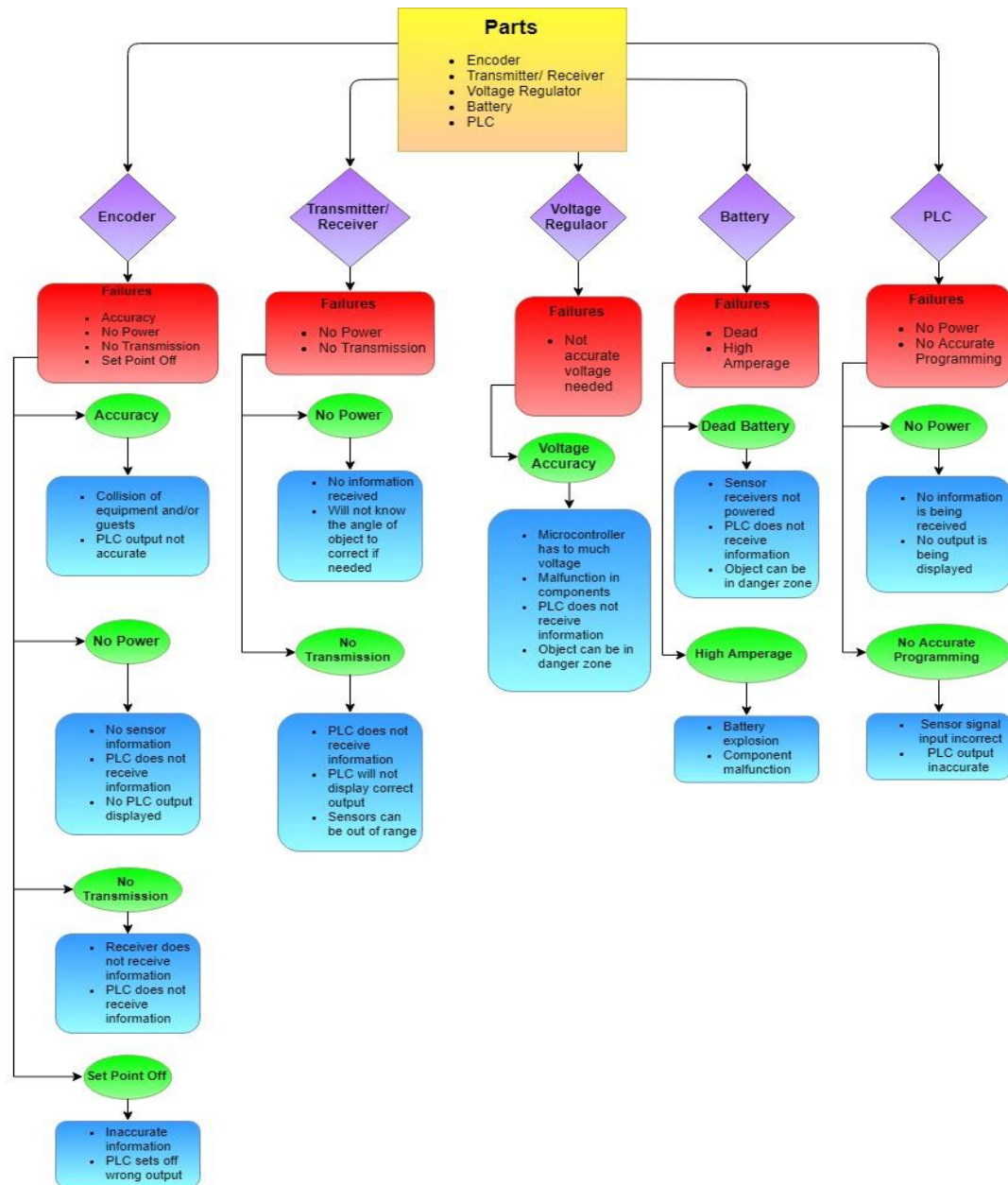
Figure 34: Failure Modes and Effects Analysis (FMEA)
