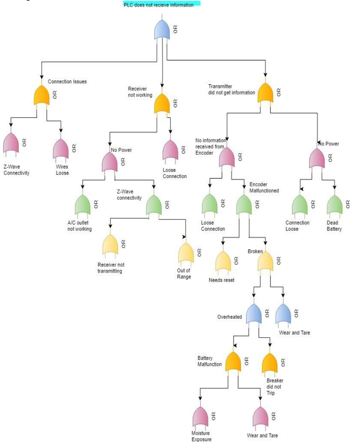
Figure 33: Fault Tree Analysis of Problems
