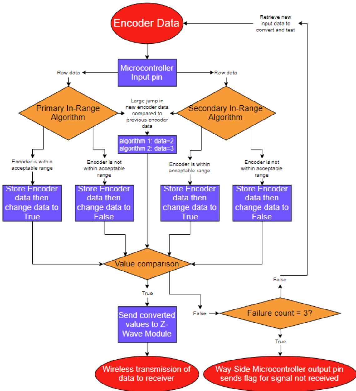
Figure 35: On-board failsafe code flow diagram
