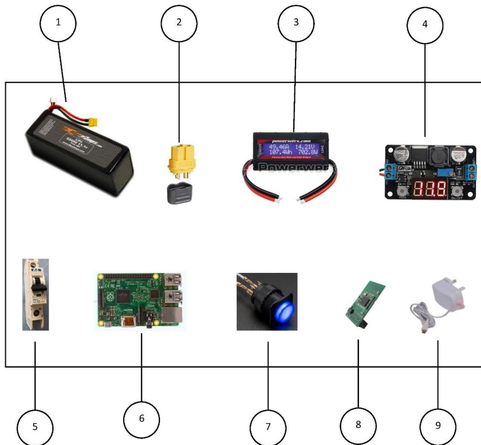
Figure 22: On-Board Control Box Assembly Drawing
