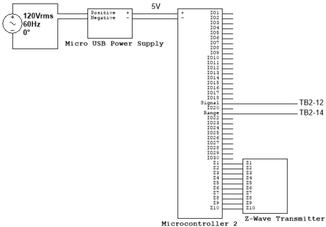
Figure 30: Track Side Box Schematic
